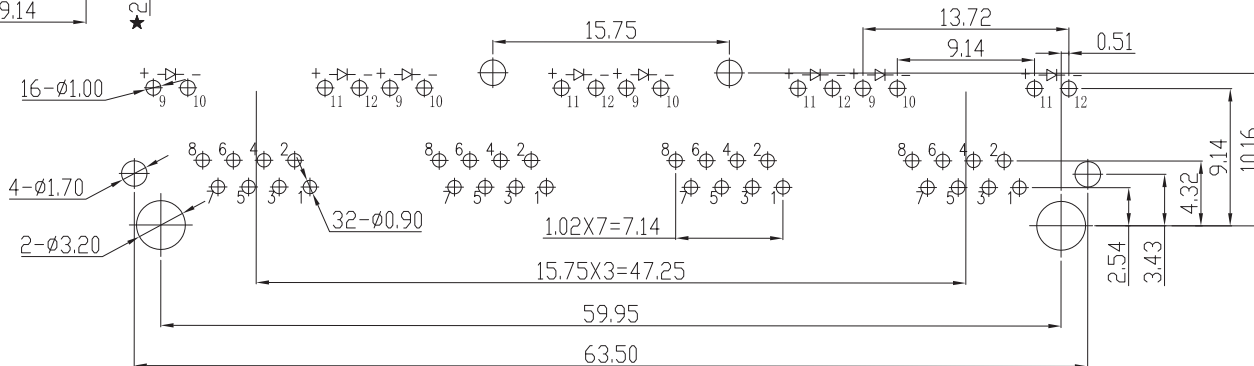
PC Board Layout
