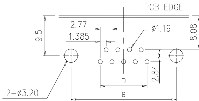
PCB layout
