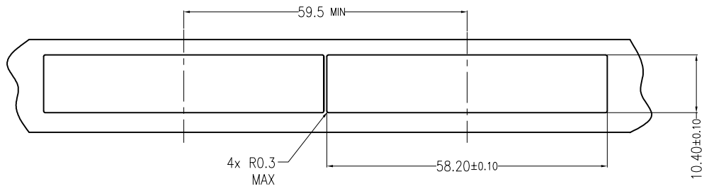
RECOMMENDED BEZEL CUT-OUT SINGLE SIDED APPLICATIONS SCALE 5:3
