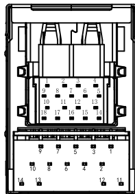
BOTTOM VIEW
