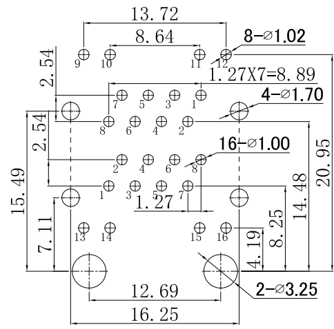
PC Board Layout
