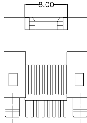
BOTTOM VIEW
