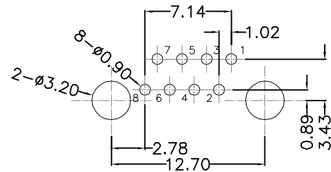
RECOMMENDED PCB LAYOUT VIEWED FROM COMPONENT SIDE
