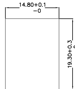
Single Panel-Latch Clearance Panel Thickness 1.60mm
