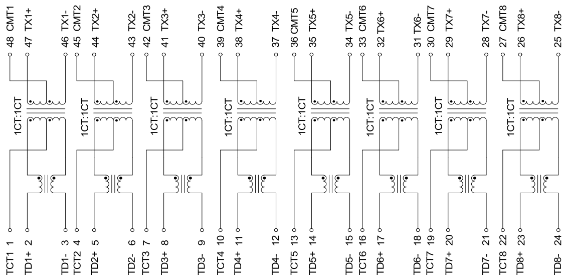
Chip Side
