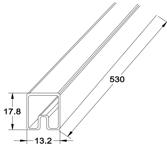
Tube: 530*13.2*17.8mm
