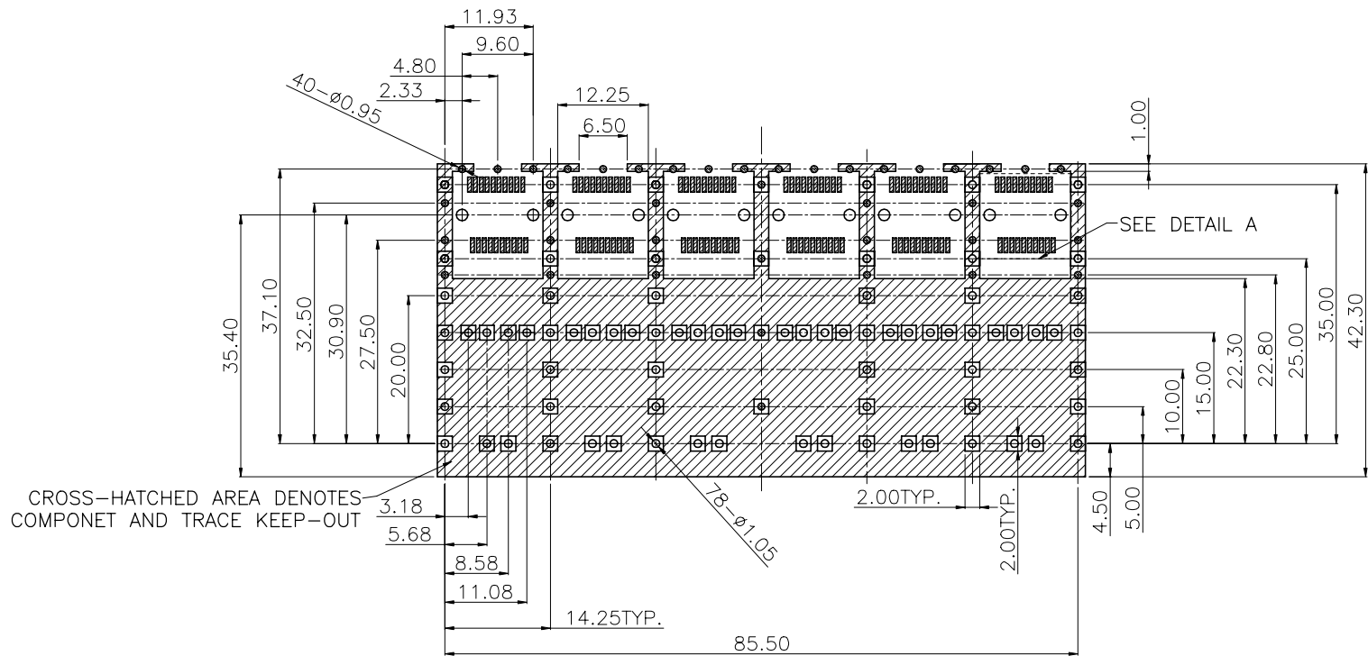
RECOMMENDED PCB LAYOUT (COMPONENT SIDE)
