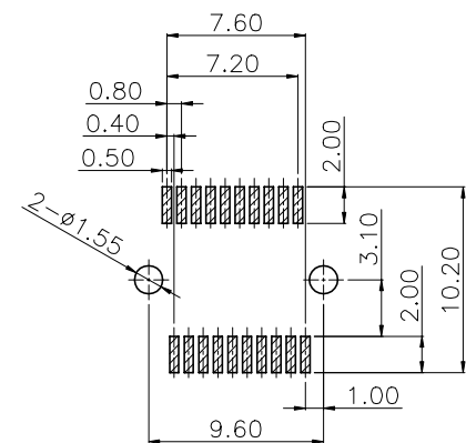
DETAIL A(SCALE 2:1)
