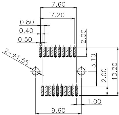
DETAIL A(SCALE 2:1)
