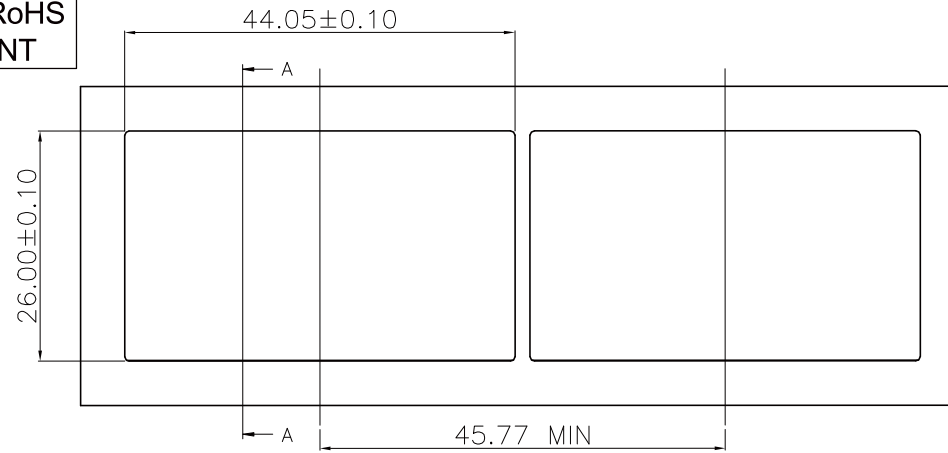
RECOMMENDED PANEL CUTOUT AND PC BOARD POSITION AND THICKNESS 0.8-2.6
