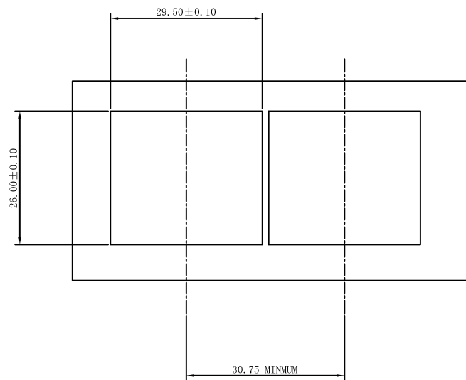
BEZEL CUT-OUT CENTER SPACING DETAIL BZZEL THICKNESS:0.8-2.6
