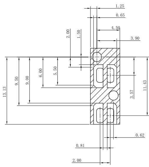
DETAIL SCALE 5:1
