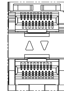
LIGHT PIPES
