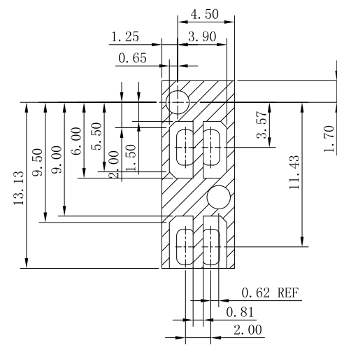
KEEP-OUT ZONE DETAIL SCALE 5:1
