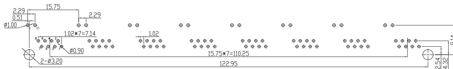
PC Board Layout
