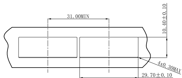
RECOMMENDED BEZEL CUT-OUT SINGLE SIDED APPLICATIONS
