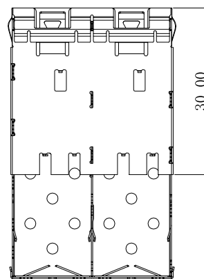
VIEW A
