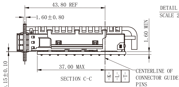
PCB LAYOUT FOR SINGLE SIDED APPLICATION
