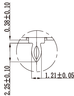
DETAIL A SCALE 4:1 QUANTITY:6
