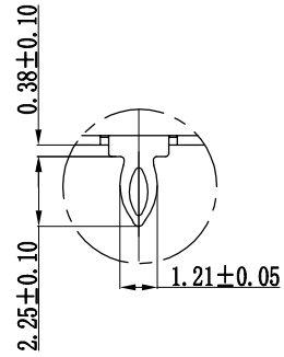
DETAIL A SCALE 4:1 QUANTITY:6
