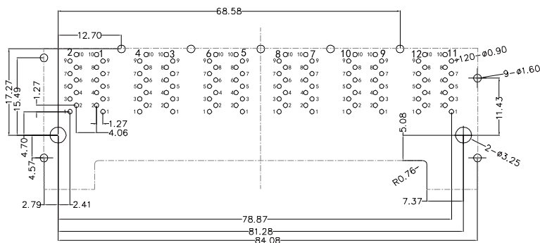
RECOMMENDED PCB LAYOUT VIEWED FROM COMPONENT SIDE
