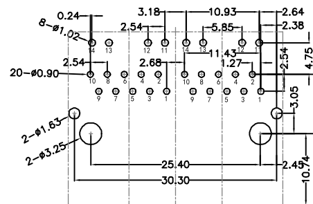
RECOMMENDED PCB LAYOUT VIEWED FROM COMPONENT SIDE
