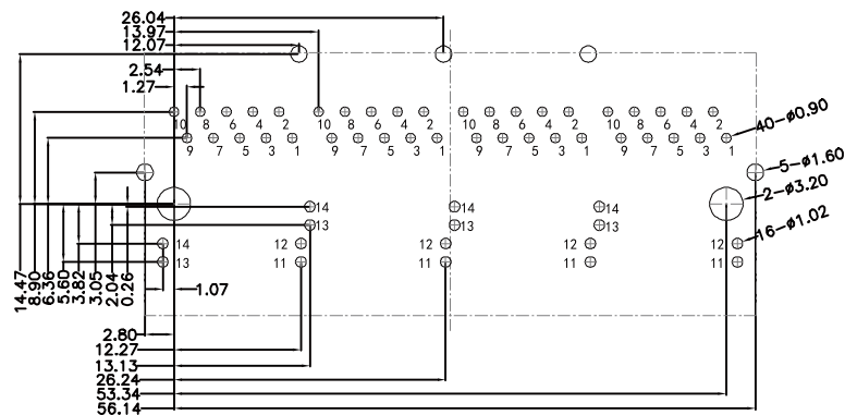
RECOMMENDED PCB LAYOUT VIEWED FROM COMPONENT SIDE
