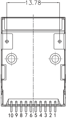
BOTTOM VIEW
