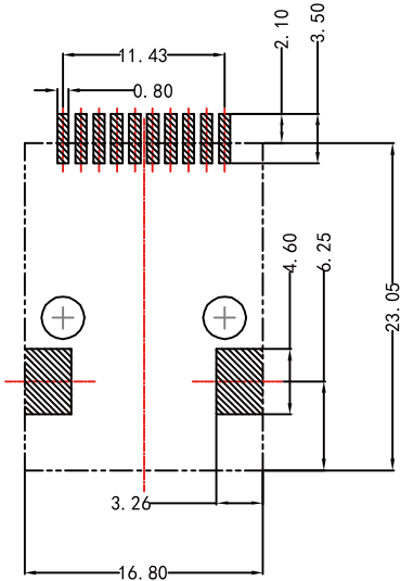
Recommended PWB Layout (Component Side View):
