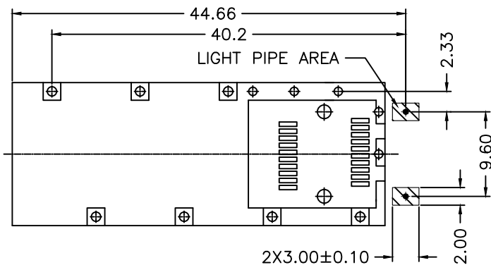
ECOMMENDED PCB CONFIGURATION
