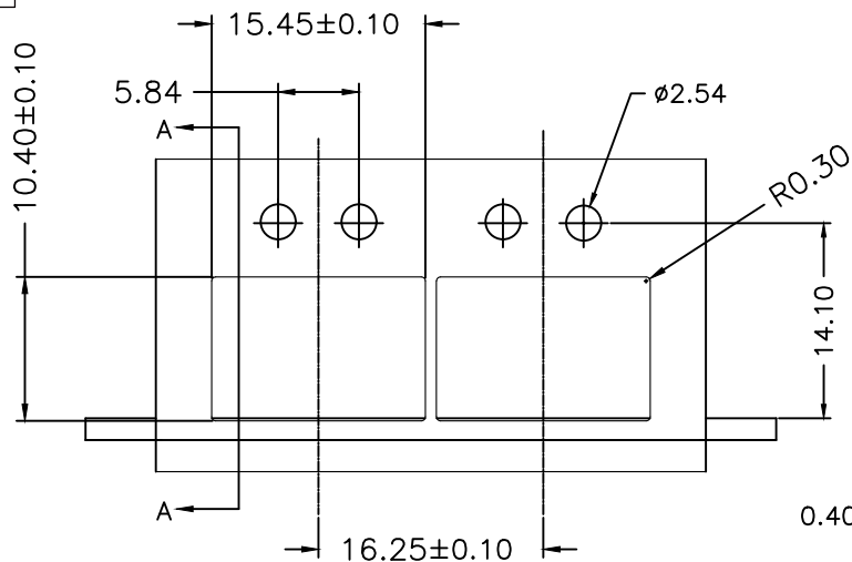
RECOMMENDED BEZEL DESIGN
