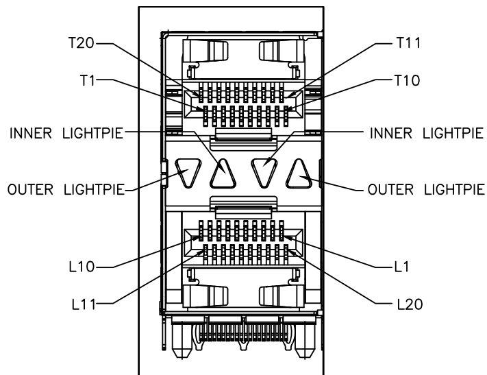
DETAIL A CIRCUIT NUMBERING AND LIGHTPIE IDENTIFICATION
