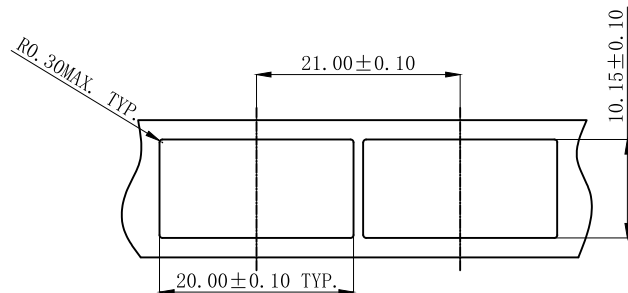
RECOMMENDED BEZEL DESIGN
