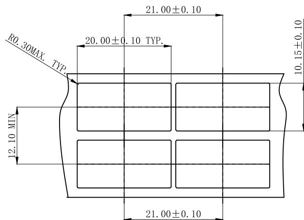
RECOMMENDED BEZEL CUT-OUT BELLY TO BELLY APPLICATIONS
