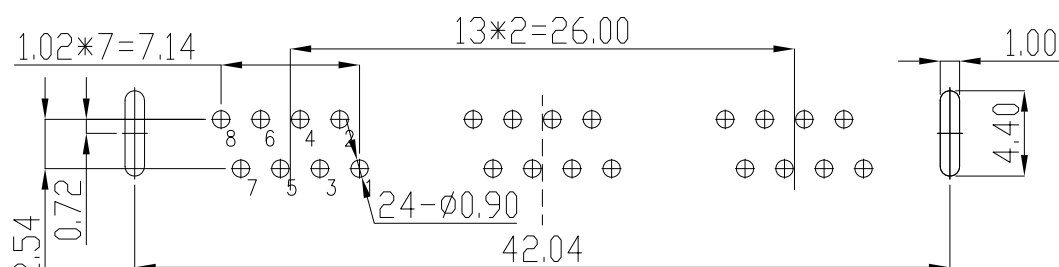
PC Board Layout
