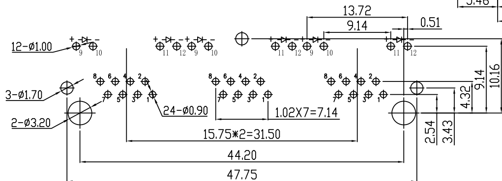
PC Board Layout
